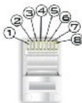
RJ45 (Plug) Cable Head
